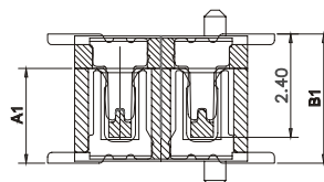
Mating Draw (Ref)
