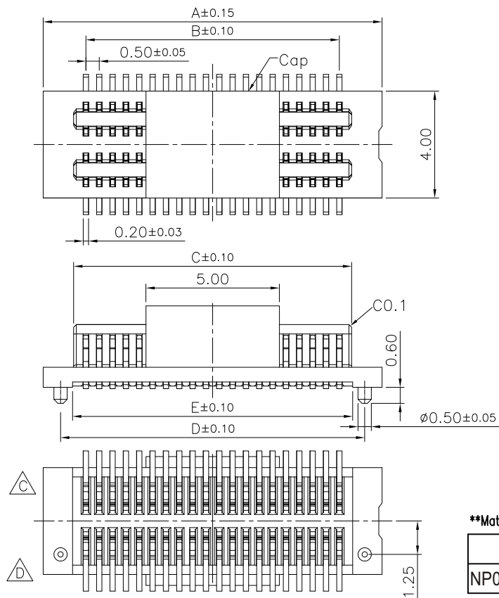
Mating Drawing (Ref)
