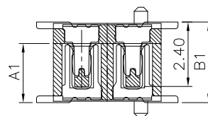
Mating Drawing (Ref)
