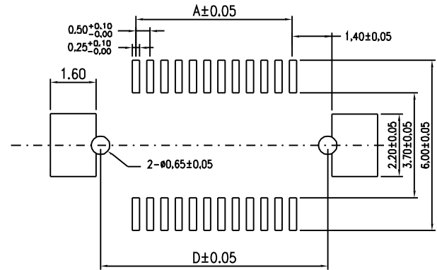
Reconnended P.C.Board Hole Layout
