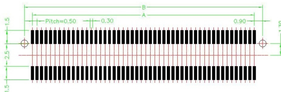
PCB Layout For Surface Mounting
