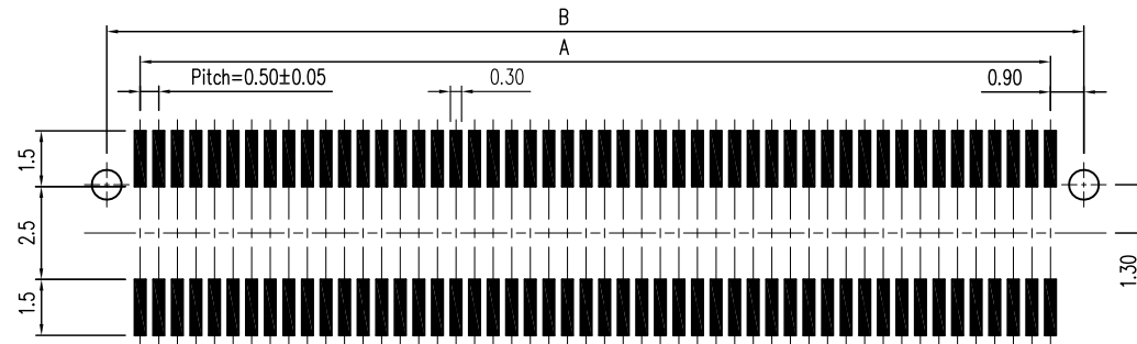
PCB Layout For Surface Mounting
