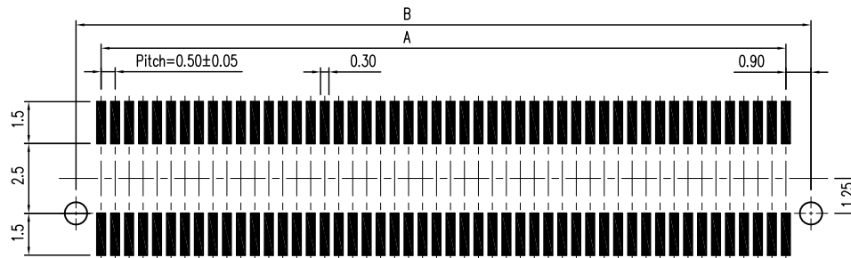
PCB Layout For Surface Mounting
