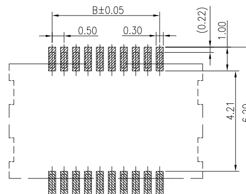
RECOMMENDED PCB PATTERN DIM. TOLERANCE : ±0.05
