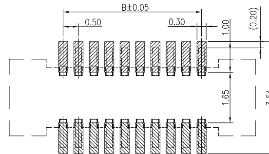
RECOMMENDED PCB PATTERN DIM.
