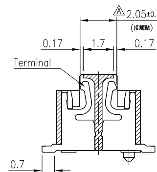
SEC. X-X
