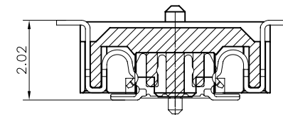
MATING
