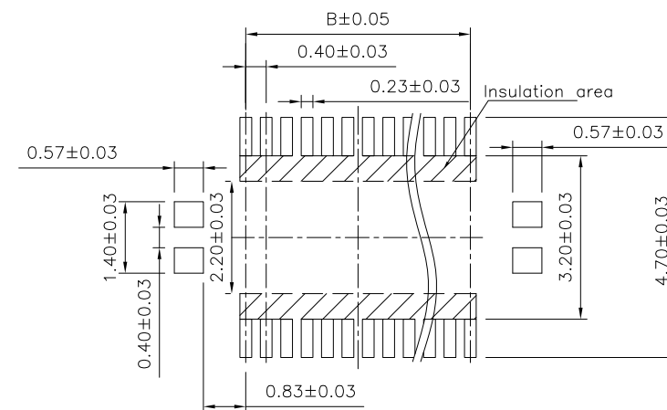
PCB Layout
