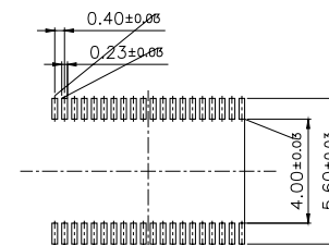
Recommended PC board pattern (Scale 5:1)
