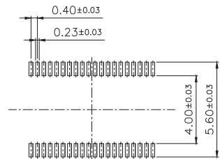
Recommended PC board pattern (Scale 5:1)
