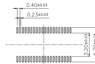
Recommended PC board pattern (Scale 5:1)
