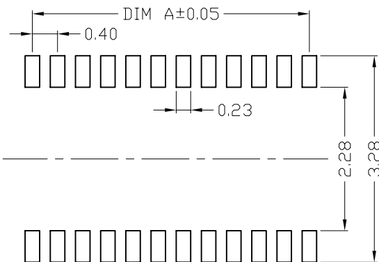
RECOMMENDED PCB LAYOUT CONNECTOR SIDE
