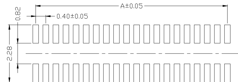
RECOMMENDED PCB LAYOUT CONNECTOR SIDE
