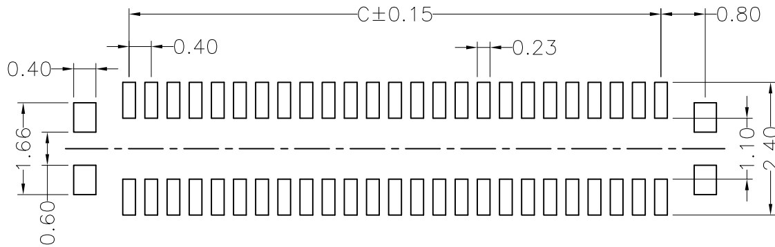
RECOMMENDED PCB LAYOUT CONNECTOR SIDE
