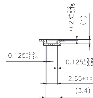
SECTION B-B (Scale 2:1)
