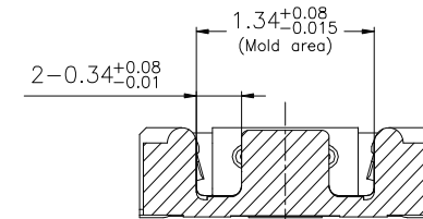
SECTION B-B (Scale 20:1)
