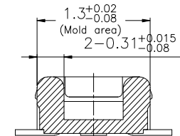
SECTION B-B (Scale 20:1)
