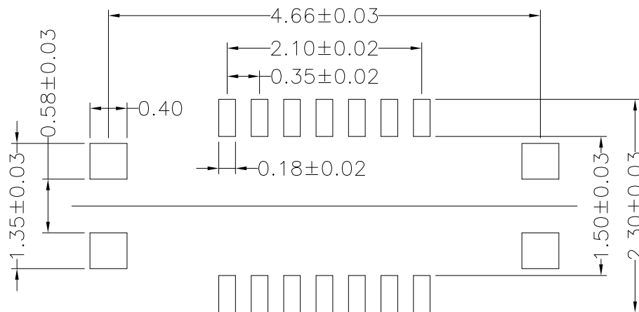
RECOMMENDED PCB LAYOUT CONNECTOR SIDE
