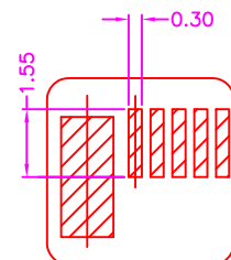
DETAIL B SCALE 2:1
