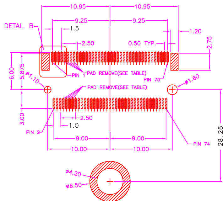
P.C.B. LAYOUT TOP VIEW \pm 0.05
