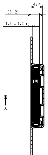
SECTION B-B
