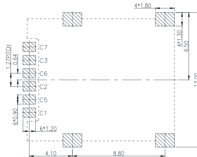
Unit: mm; Tolerances: \pm 0.05 mm Figure 5.2 Reference dimension for PCB layout
