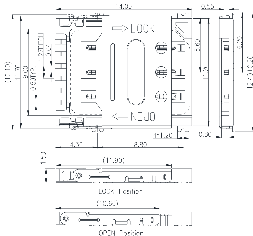
Unit: mm; Tolerances: \pm 0.15 mm Figure 5.1 Mechanical outline dimension
