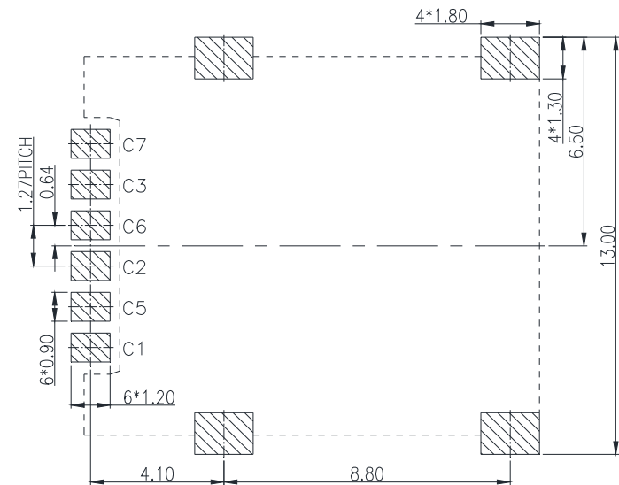
Unit: mm; Tolerances: \pm 0.05 mm Figure 5.2 Reference dimension for PCB layout
