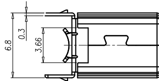
FRONT SHELL
