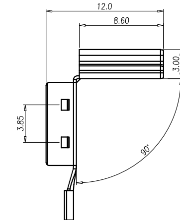
FRONT SHELL
