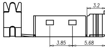
FRONT SHELL
