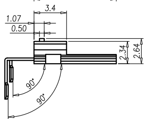
HOUSING+PIN
