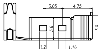
BACK SHELL
