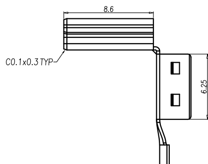
FRONT SHELL
