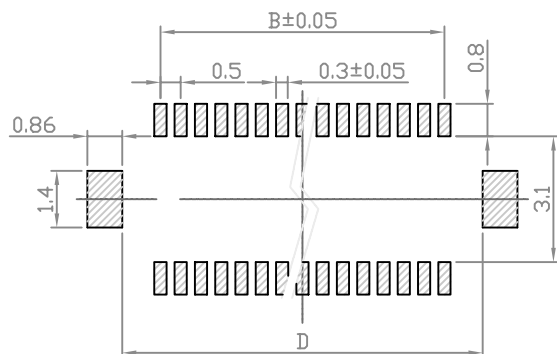
RECOMMEND PCB LAYOUT (COMPONENT SIDE)
