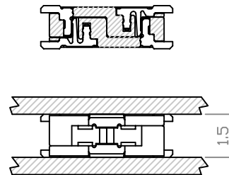
MATED DRAWING
