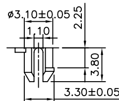
DETAIL X
