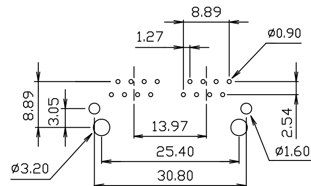
PC Board Layout Ref.
