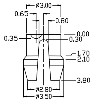
DETAIL X
