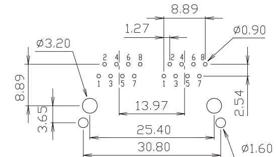
PCB LAYOUT Ref.
