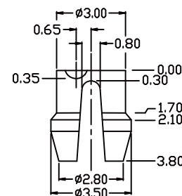
DETAIL X
