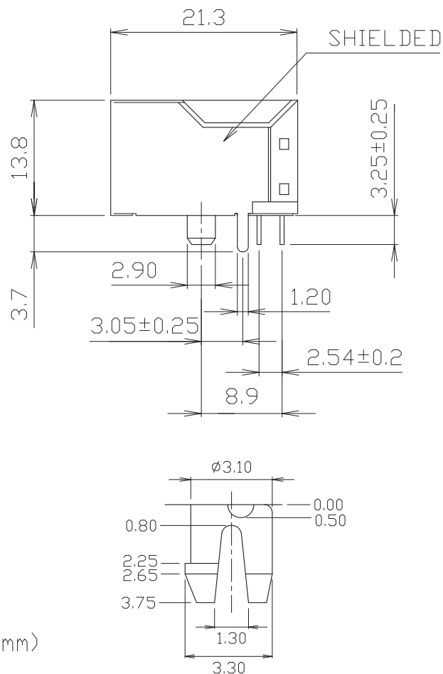
DETAIL X
