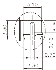
DETAIL Z SCALE 2:1
