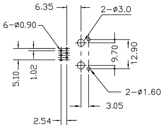
PCB LAYOUT/TOP VIEW MJF12-KX06A3-0606
