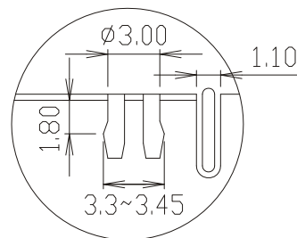
DETAIL X
