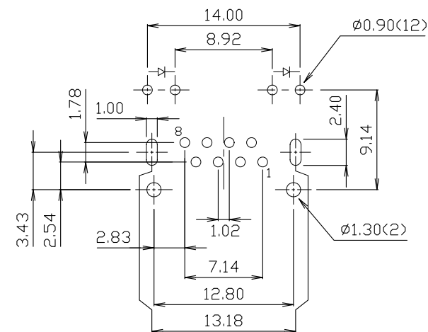
PCB LAYOUT Ref.
