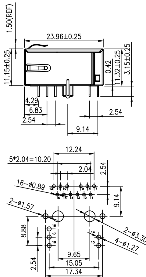
RECOMMENDED PCB LAYOUT COMPONENT SIDE
