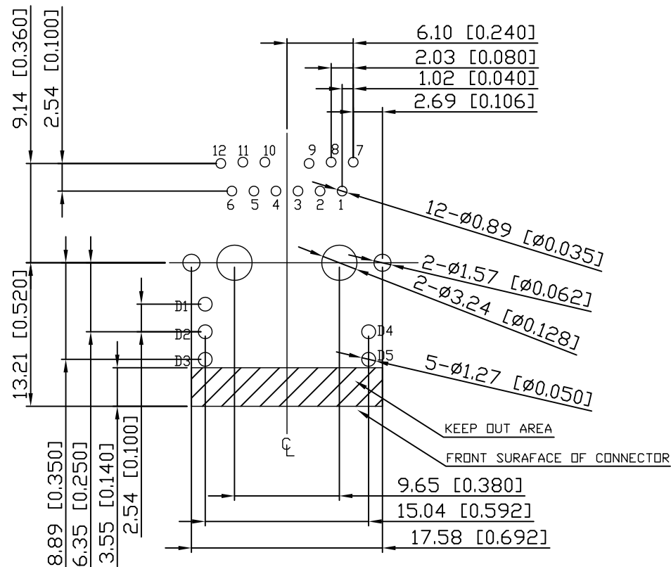
SUGGESTED PCB LAYOUT (TOP VIEW)
