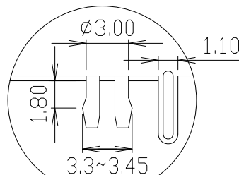
DETAIL X
