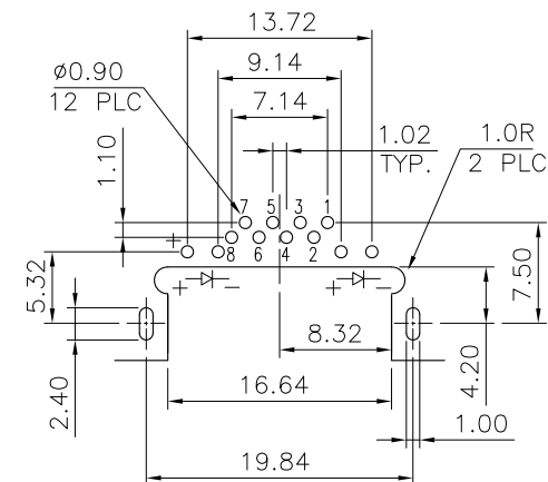
PCB LAYOUT
