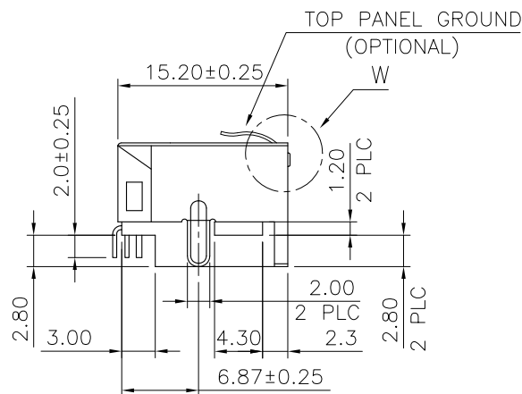
DETAIL W
