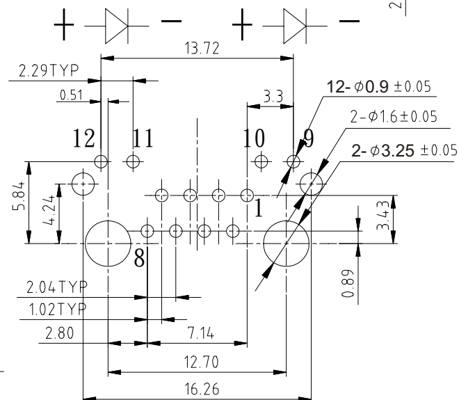
LED SCHEMATIC PCB LAYOUT/TOP VIEW
