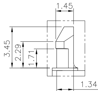
DETAIL X
