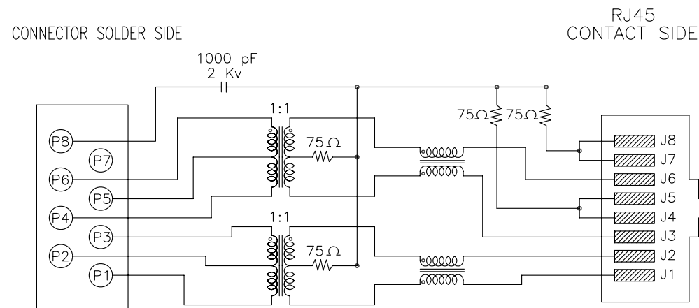
CONNECTOR SCHEMATIC
