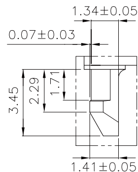
DETAIL X
