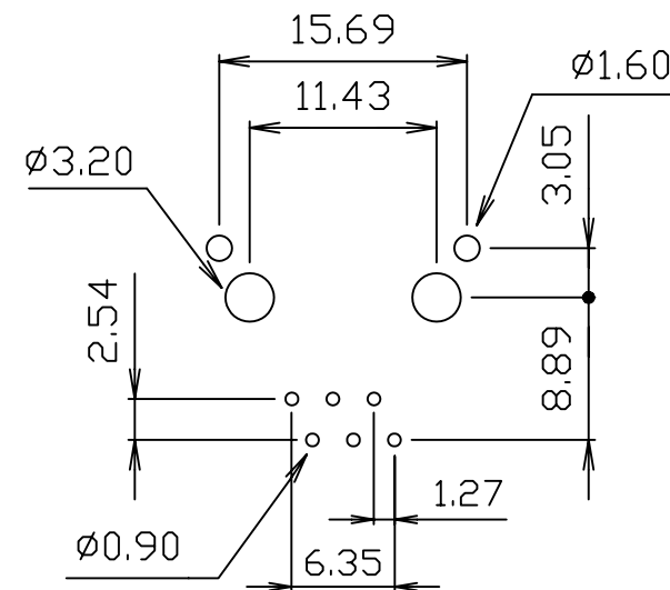
PC Board Layout
