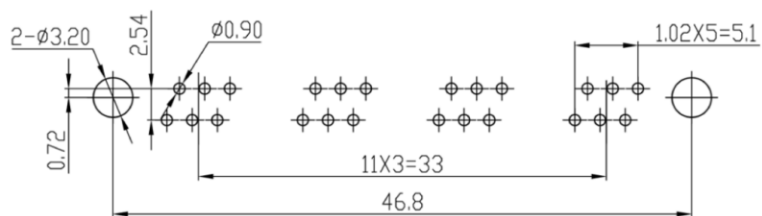
PC Board Layout
