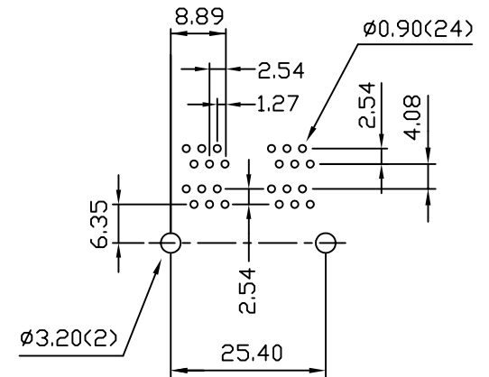
PCB LAYOUT
