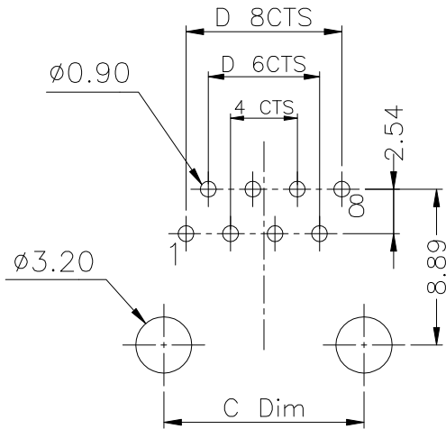
PC Board Layout PCB t=1.60mm
